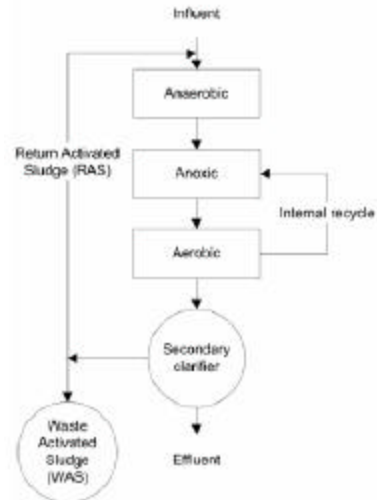
Figure 3. Anaerobic/Anoxic/Aerobic Process
